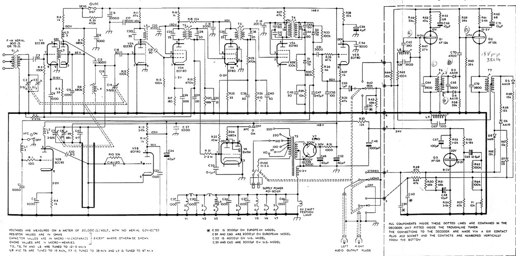
CIRCUIT DIAGRAM
