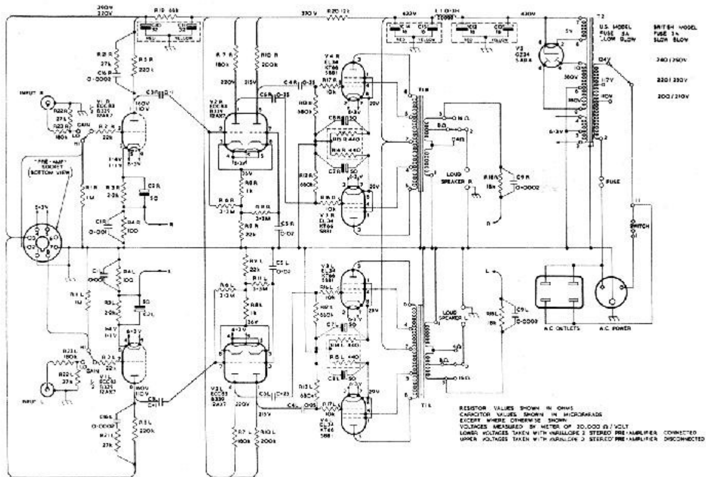
CIRCUIT DIAGRAM OF LEAK 'STEREO 60' POWER AMPLIFIER
