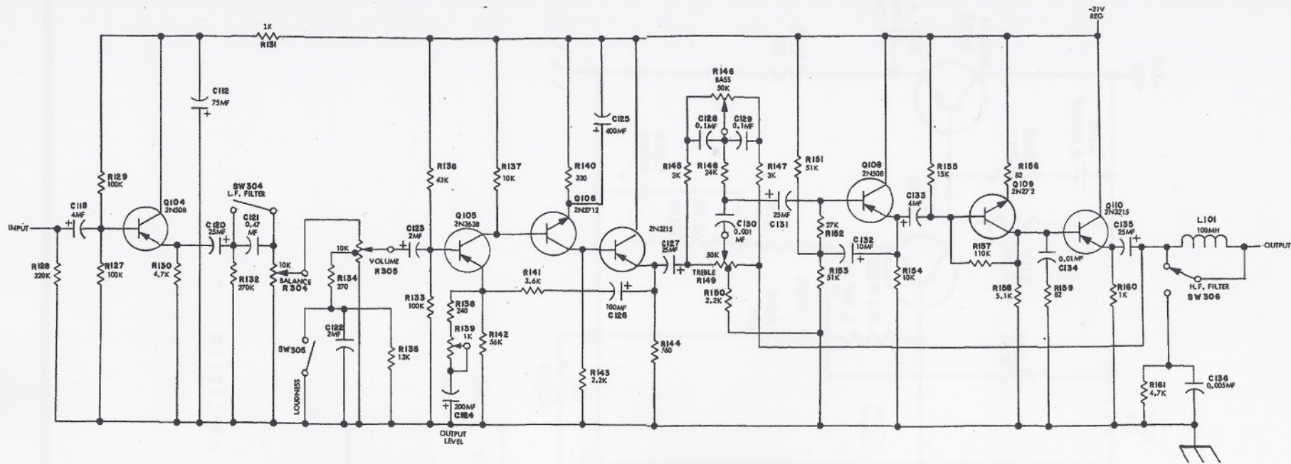
LINE AMPLIFIER
