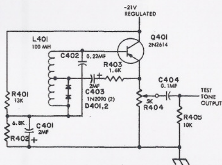
TONE OSCILLATOR
