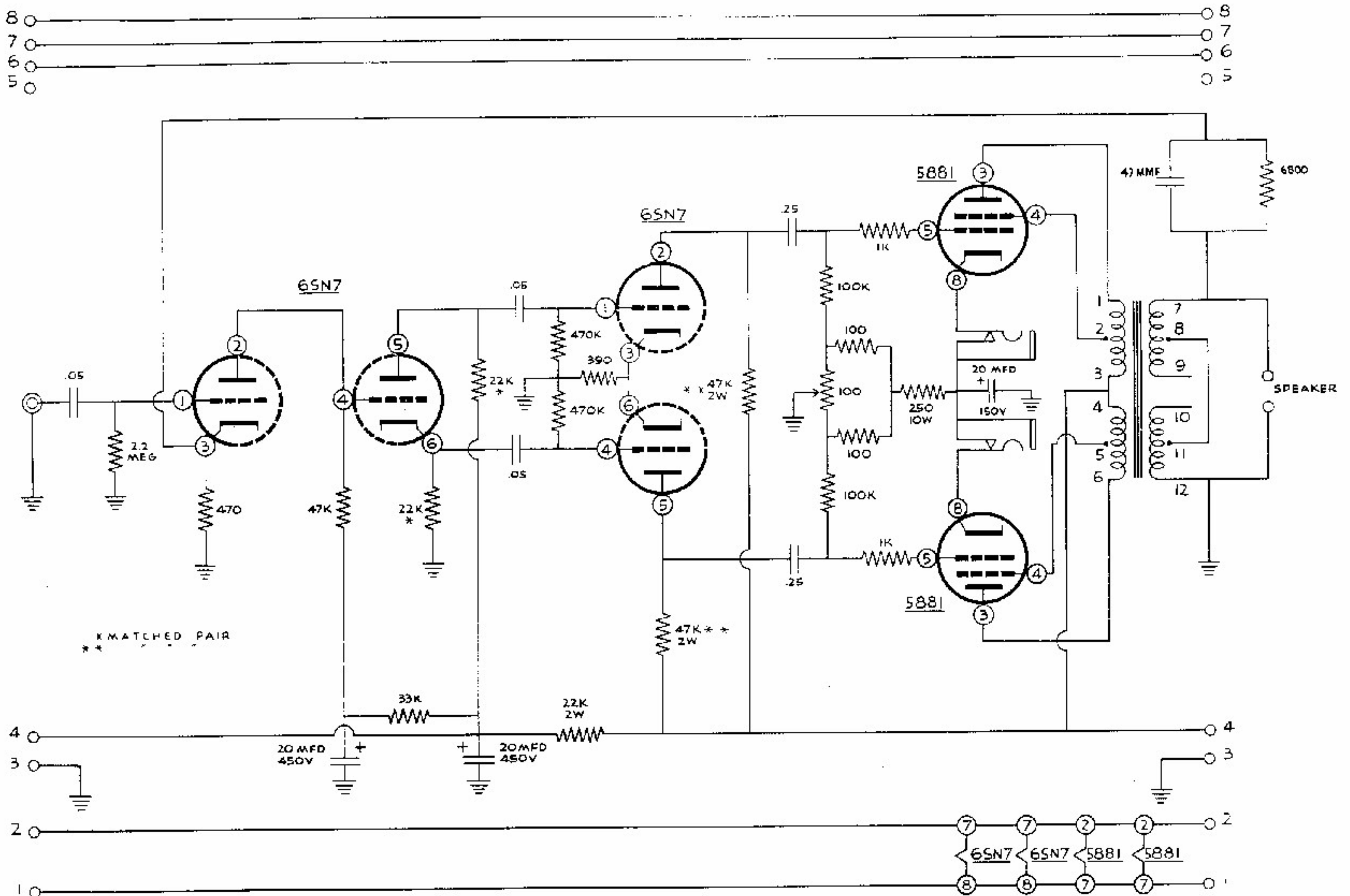
Heathkit MODEL W-2 AMPLIFIER CIRCUIT DIAGRAM
