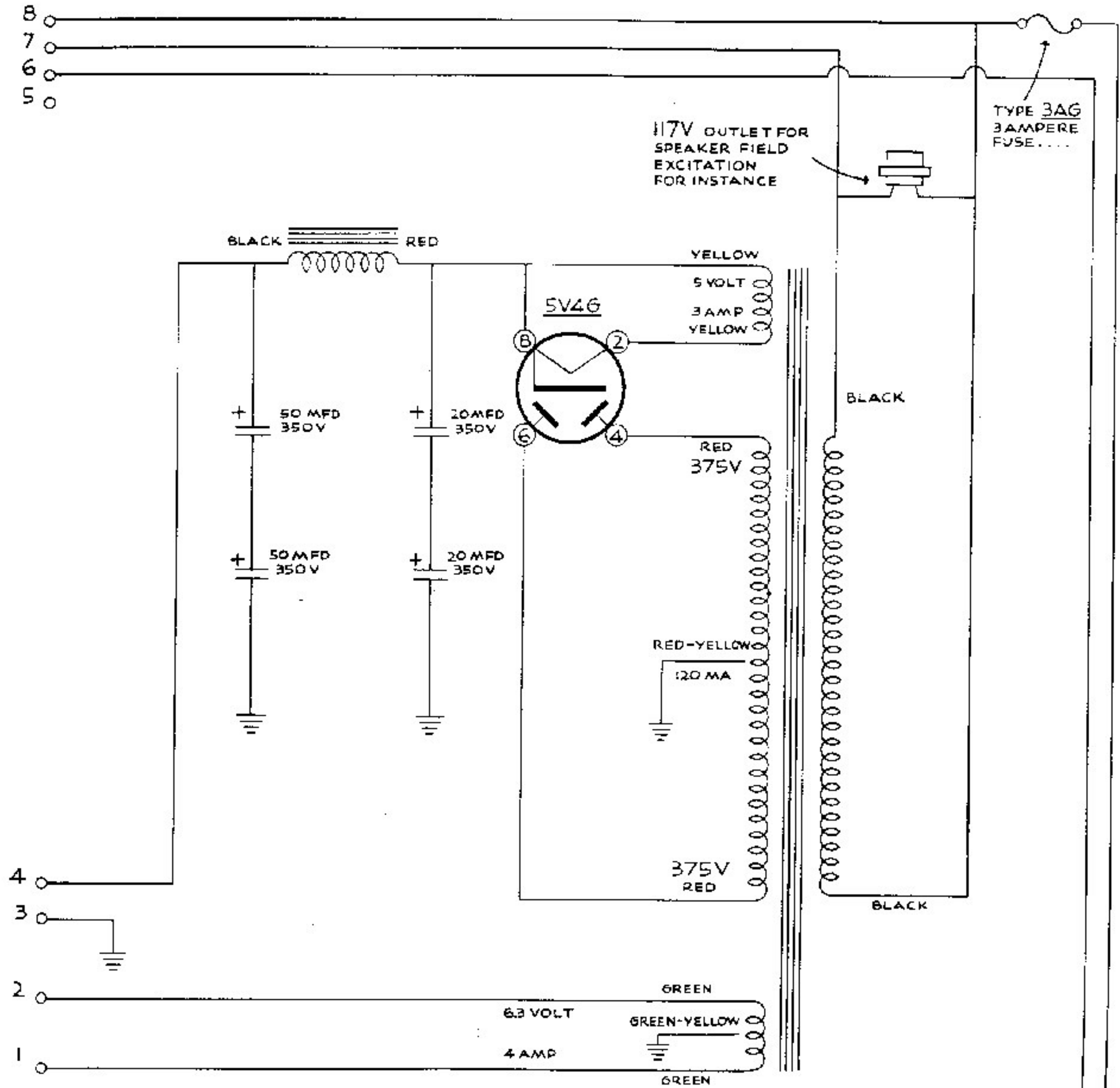
Heathkit POWER SUPPLY CIRCUIT DIAGRAM W2 Mono Amplifier
