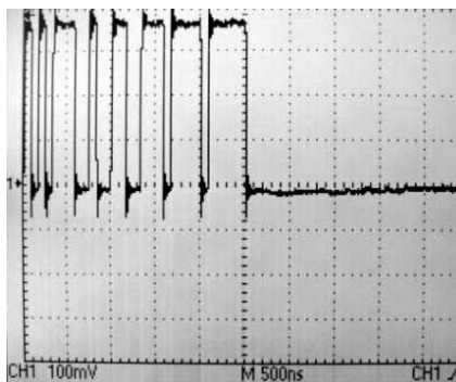
Pino 48/U3 (USBM(com pen drive conectado+MP3 ) 100,0mV/500nS/AC
