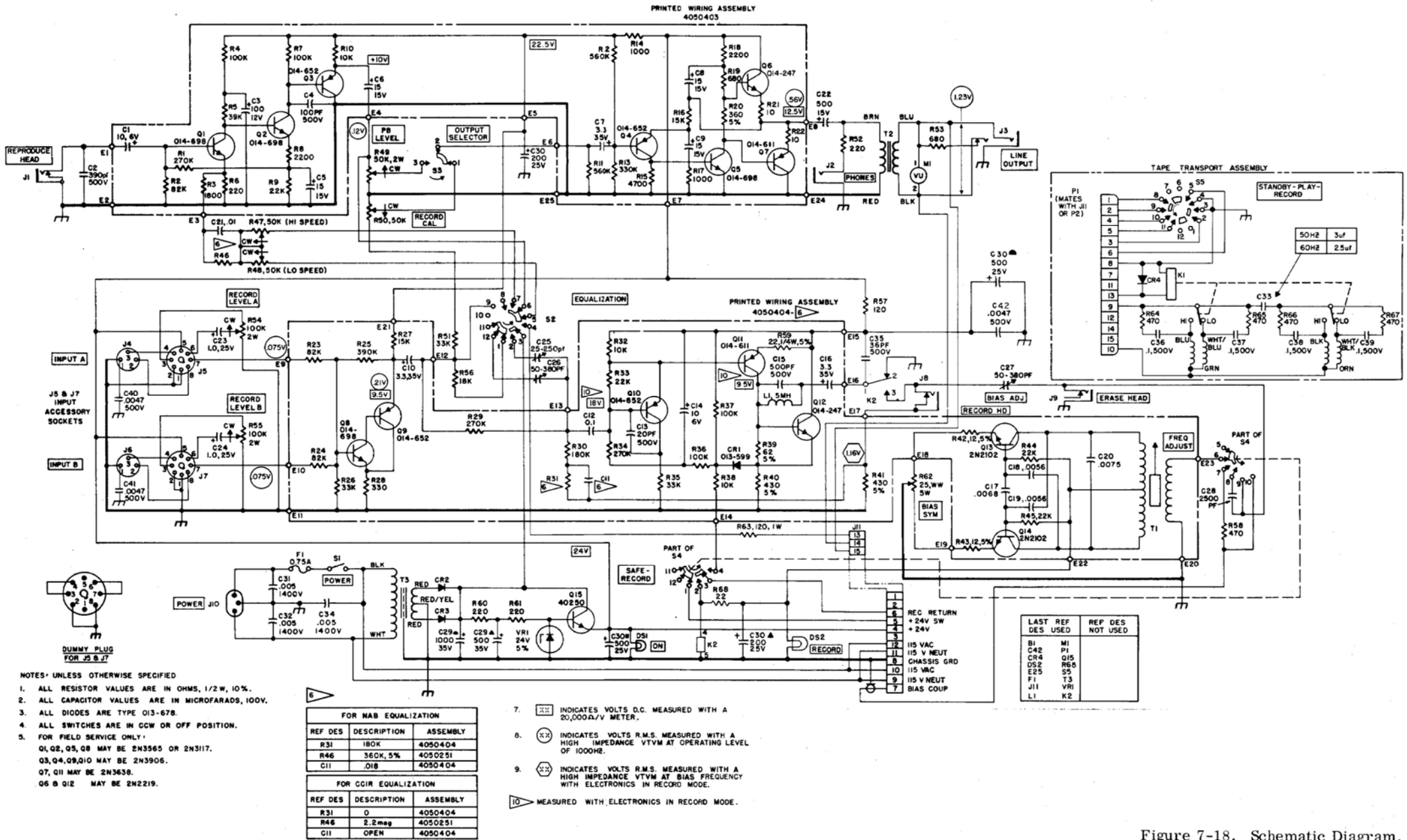
Figure 7-18. Schematic Diagram, Master Electronics (Domestic)
