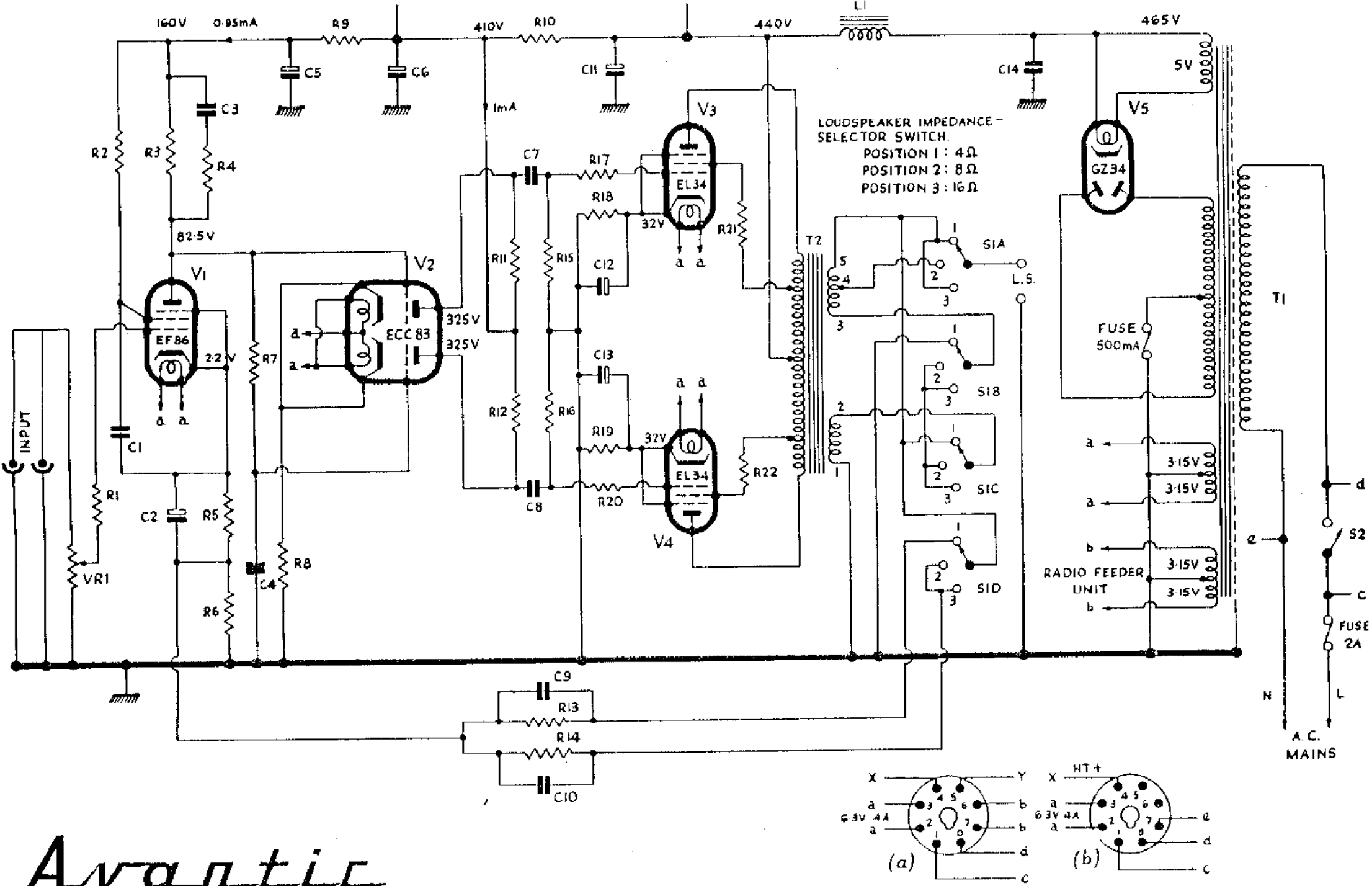
Fig. 3. Circuit diagram of power amplifier. (For component values, see page 18). Rear view of power output socket: (a) standard version (b) American version.
