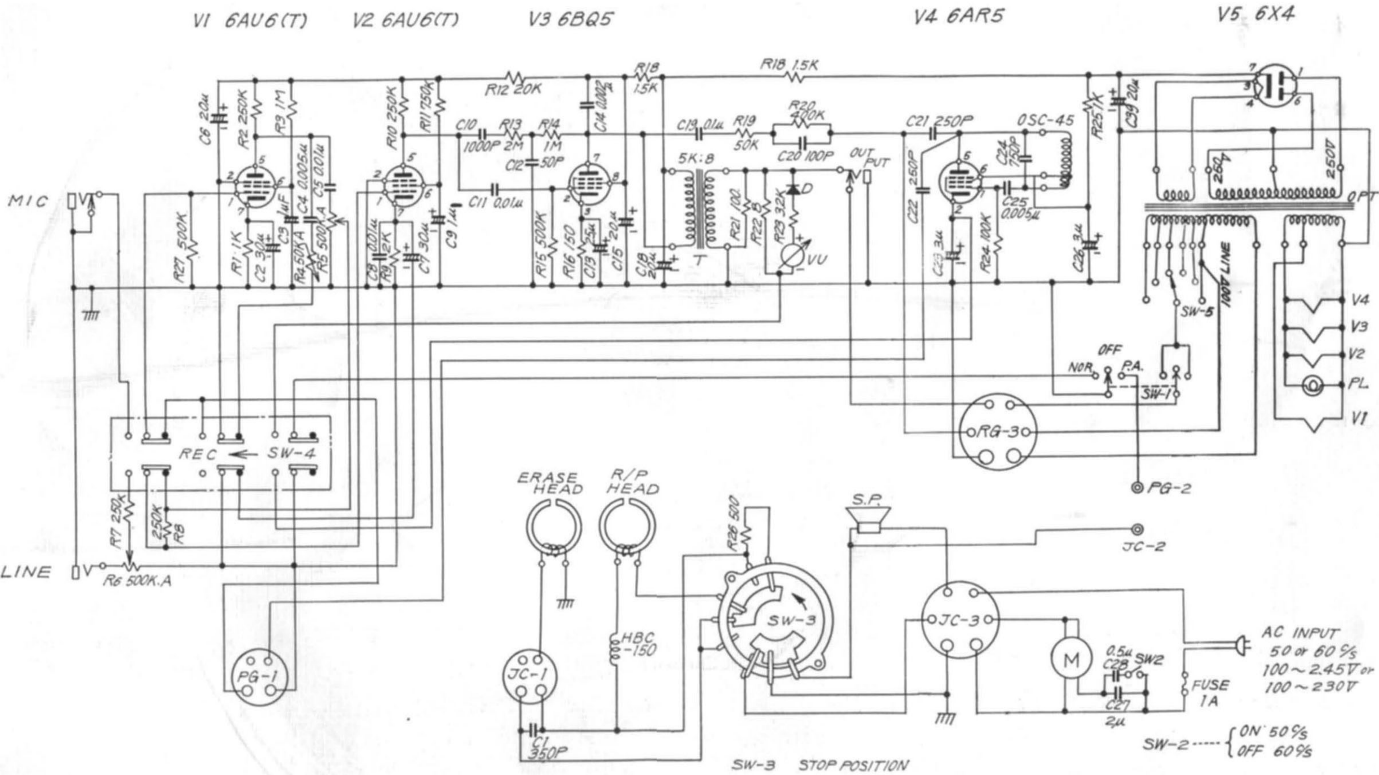
Magnetophone a bande AKAI Mod 910 (tape Recorder Reel-to-reel)
