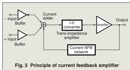
Fig. 3 Principle of current feedback amplifier
