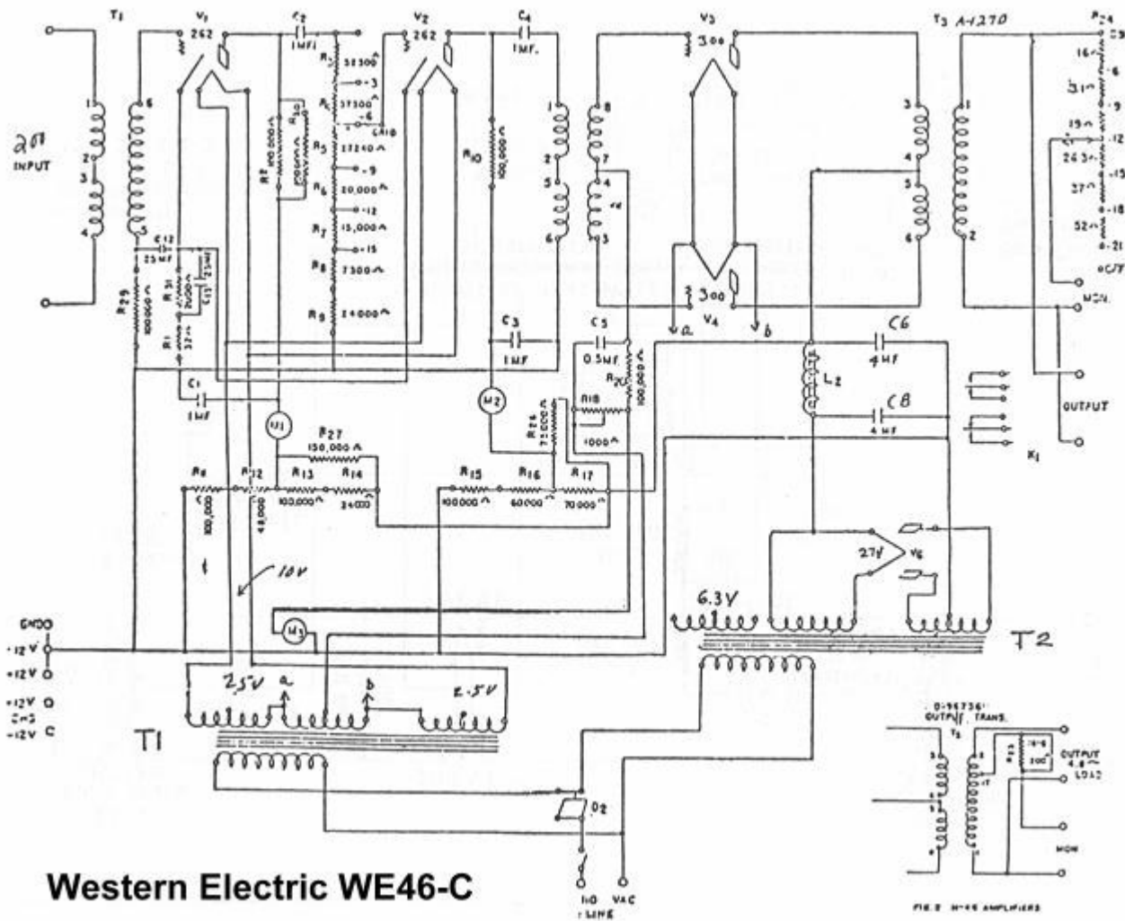
FIG. 2 WE46 AMPLIFIER
