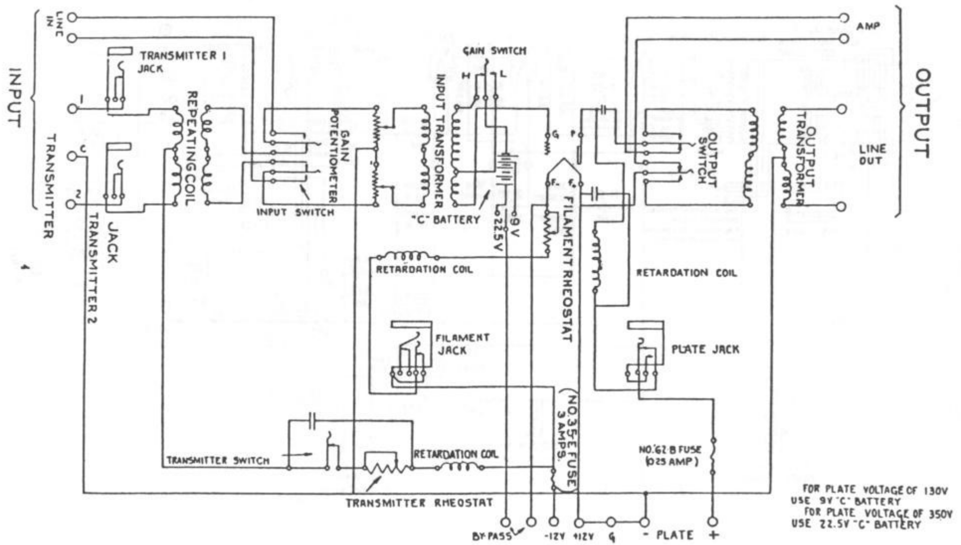
FIG. 2—CIRCUIT DIAGRAM OF NO. 11-A AMPLIFIER
