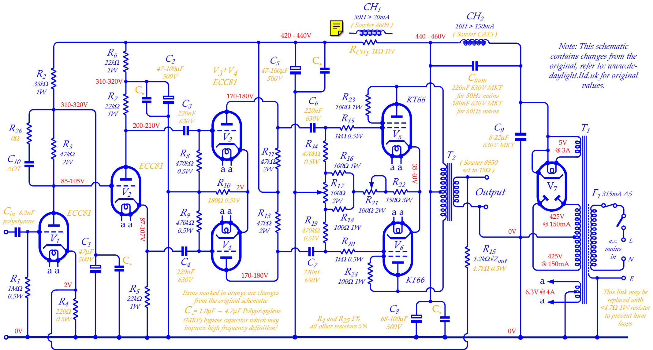
The Williamson Amplifier "new version" from Wireless World August 1949 p. 282 Redrawn 1996 by Keith Snook d.c. ~ daylight ltd.
