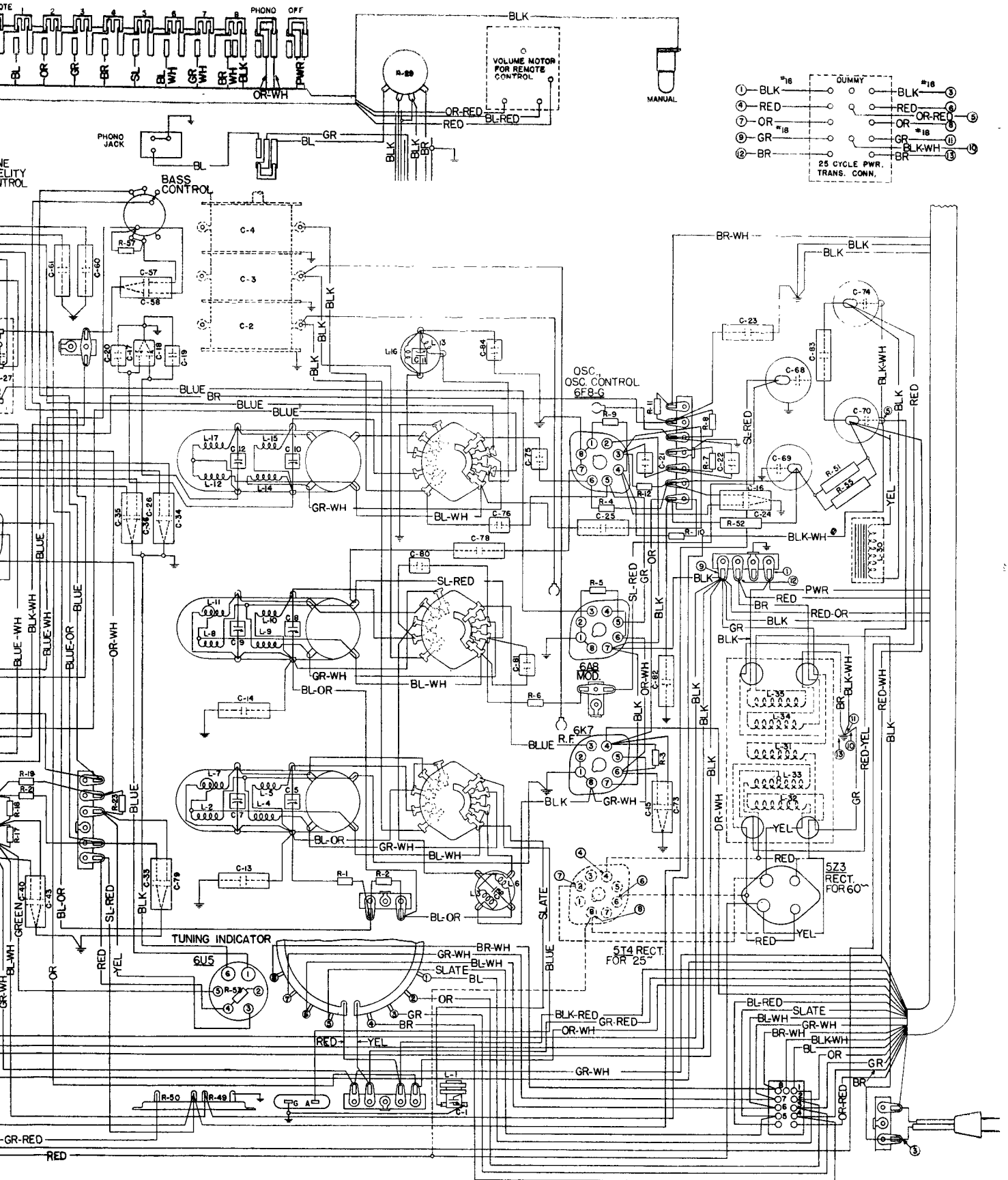
Fig. 3. Wiring Diagram of Chassis.
