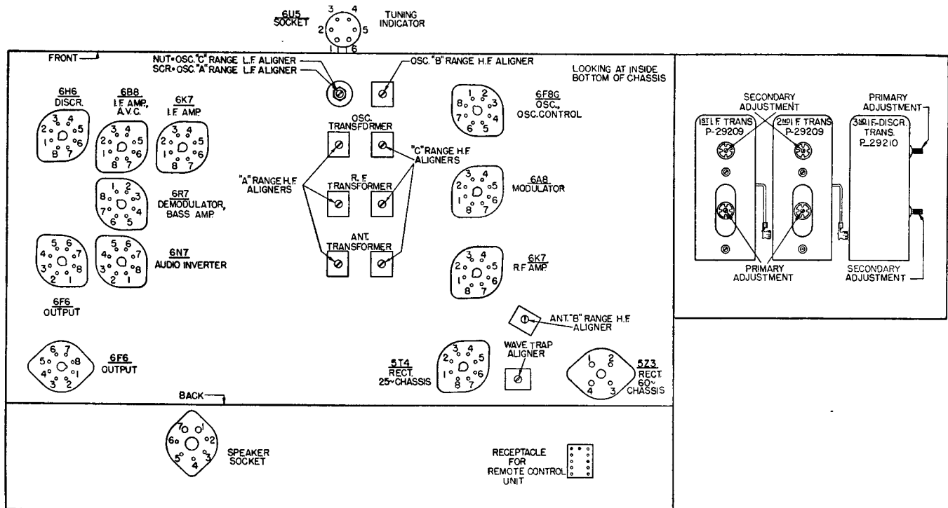
Fig. 1. Terminal Layout for Voltage Measurement Chart and Location of the Aligning Adjustments.
