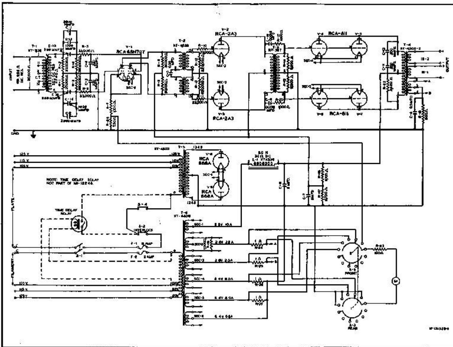
Figure 5—Schematic Diagram
