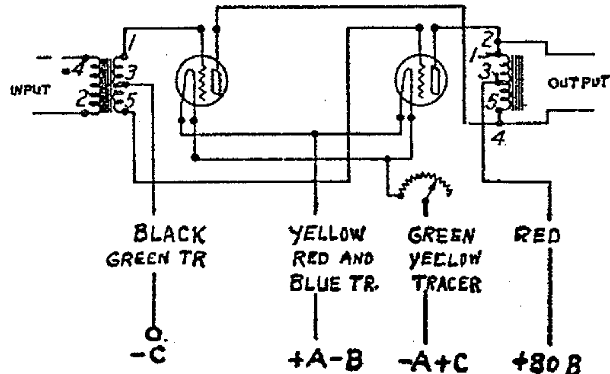
Model Radiola Balanced Amplifier (1924)
