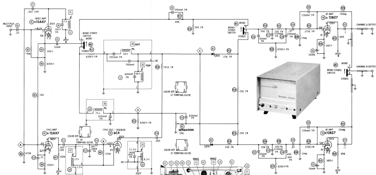
MULTIPLEX ADAPTER ALIGNMENT USING FM STEREO GENERATOR AND AUDIO GENERATOR
