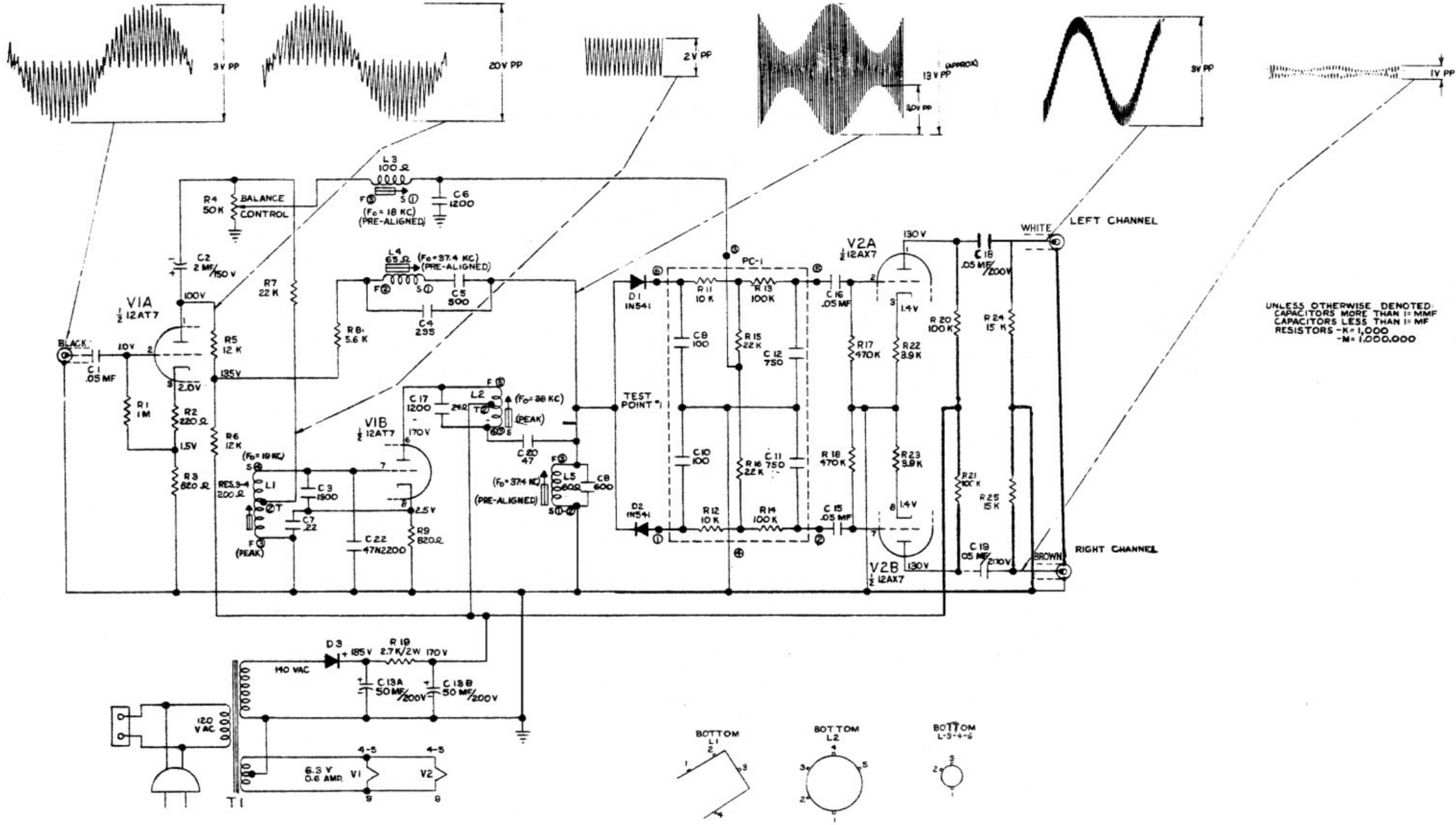
MA-2G SCHEMATIC DIAGRAM
