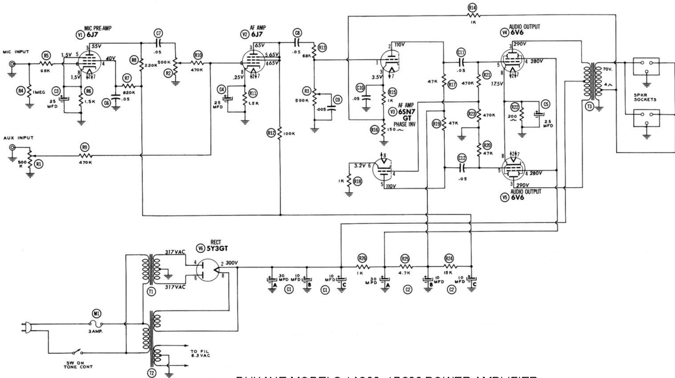
DUKANE MODELS 1A300, 1B300 POWER AMPLIFIER
