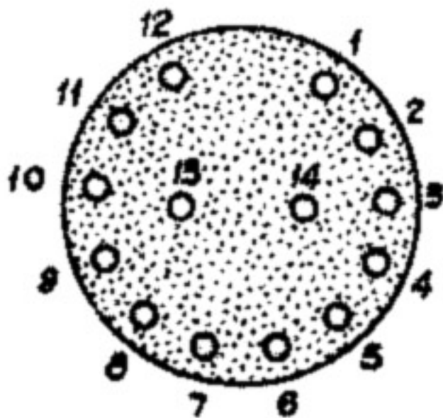
CONNECTING PLUG LOOKING AT PIN ENDS, OR SOCKET LOOKING AT REAR.
