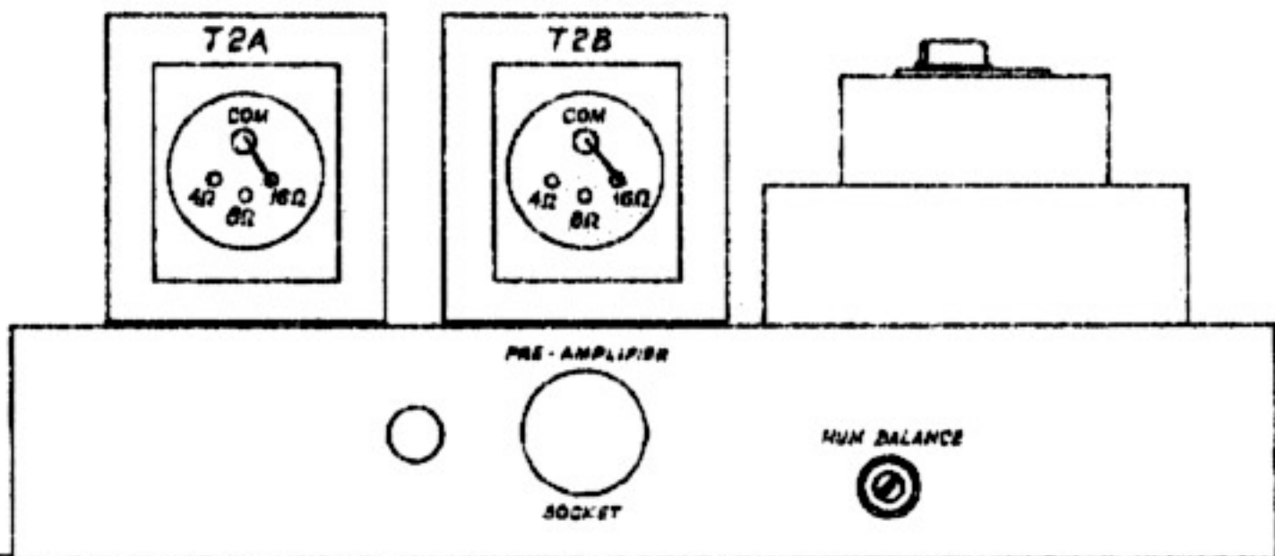
REAR VIEW
